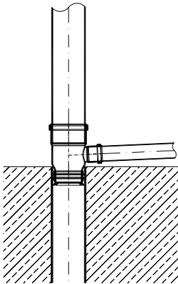
Branch inside/inside
