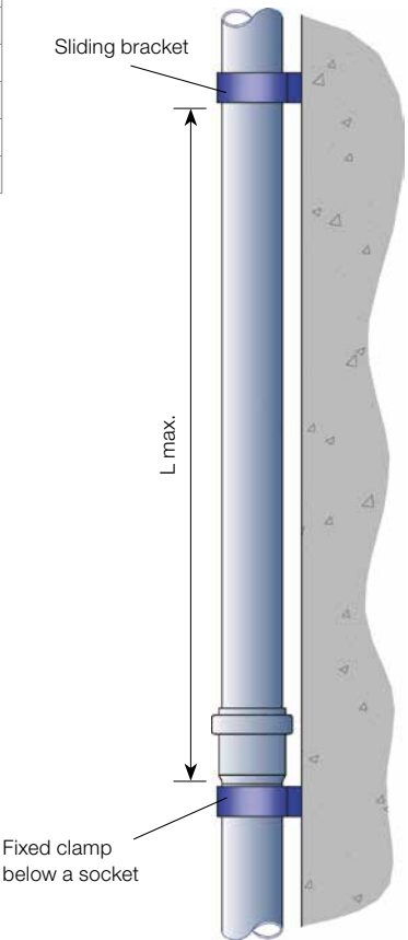
Vertical pipe routing (FIGURE 20)
