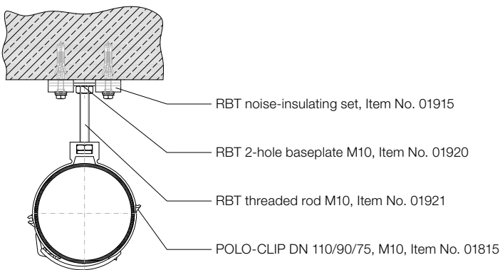
Example of noise-insulated fastening (FIGURE 13)
