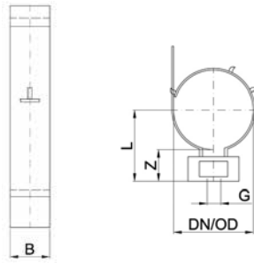
POLO-CLIP (FIGURE 9)
