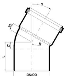
POLO-KAL NG Bend PKB with factory-fitted lip ring
