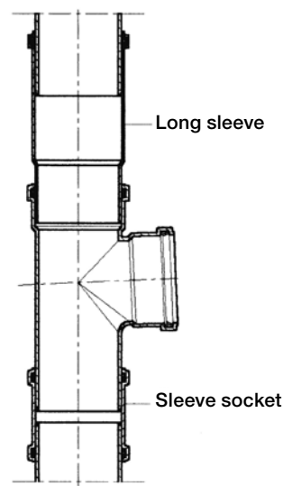
Installation of a junction with long sleeve and sleeve socket (FIGURE 30)
