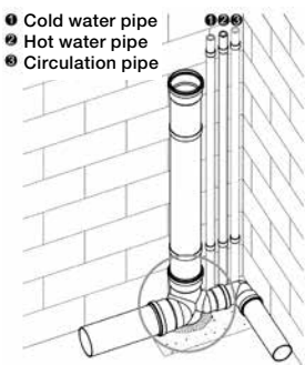
Example of installation of a bent double branch (FIGURE 32)
