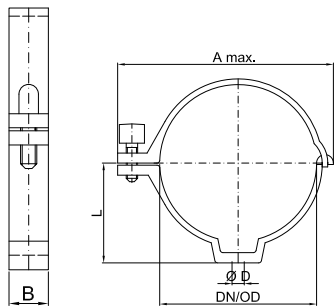
Dimensioning (FIGURE 12)
