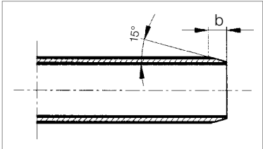
Bevelling at an angle of approx. 15° (FIGURE 18)
