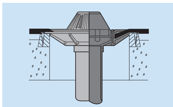
Fig.35 2171.4 Domed Outlet
