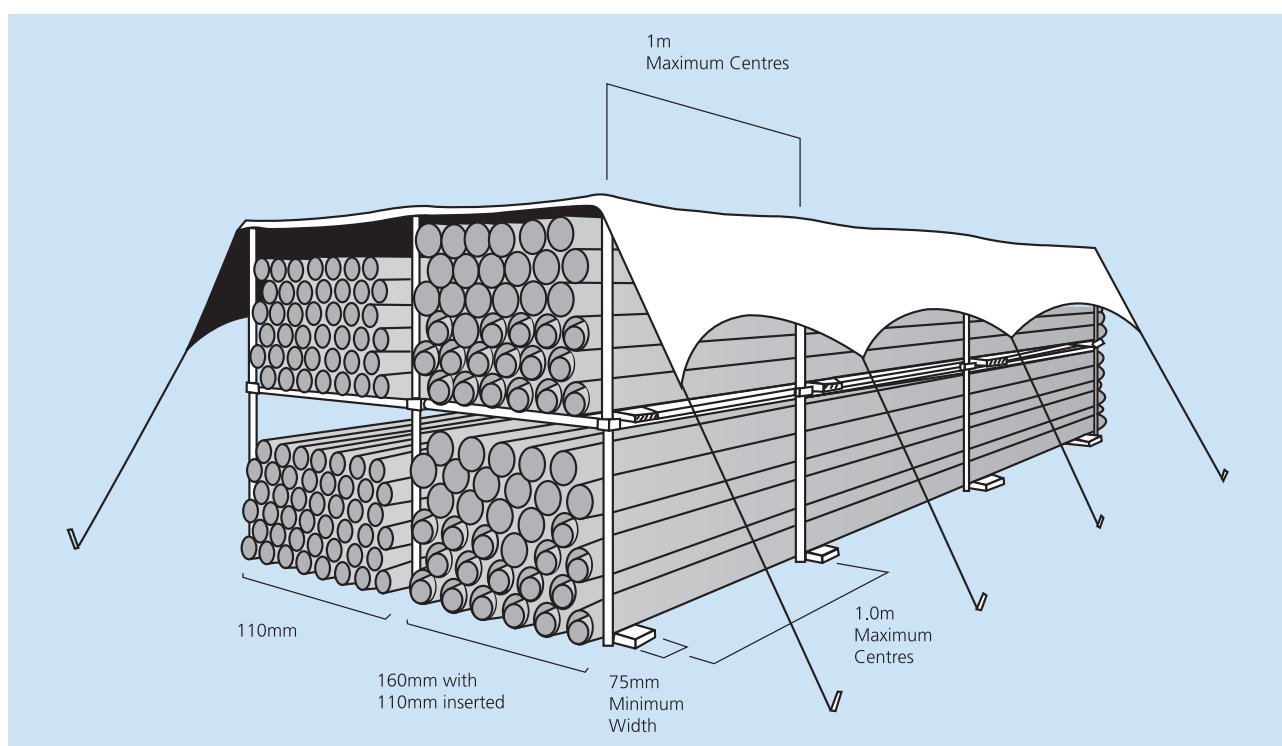
Fig. 1 Pipe stacking
