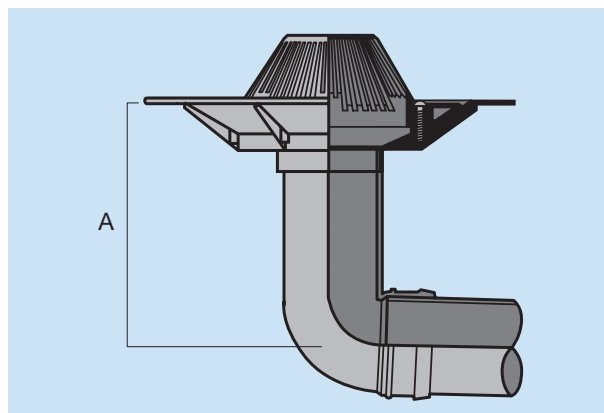
Fig.37 2171.4 Domed Outlet
