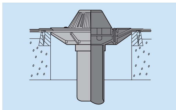
Fig.34 2171.4 Domed Outlet
